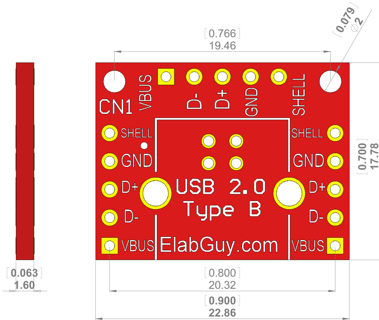
USB-BF-BO-V1A PCB Outline Drawing
